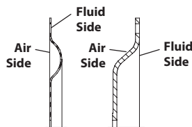
Cross Section View of Diaphragms
