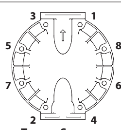
Torque Sequence
